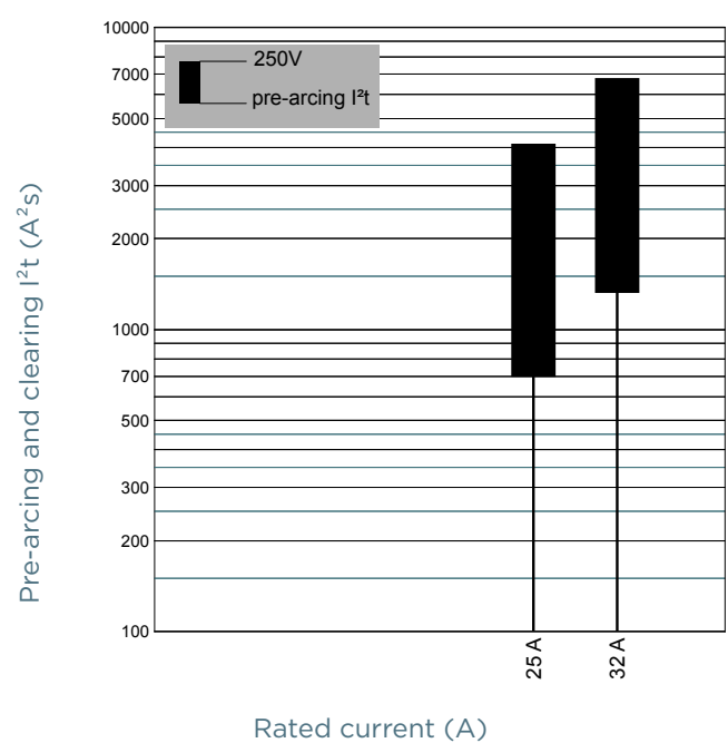
Size 10x38 250V gG with striker
