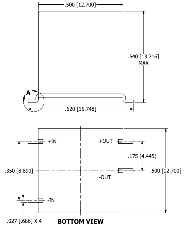
LEAD DETAILS
