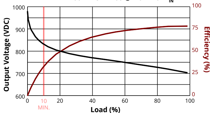
P/N 5AV1000 / 5SMV1000 @ Nominal V_{IN}
